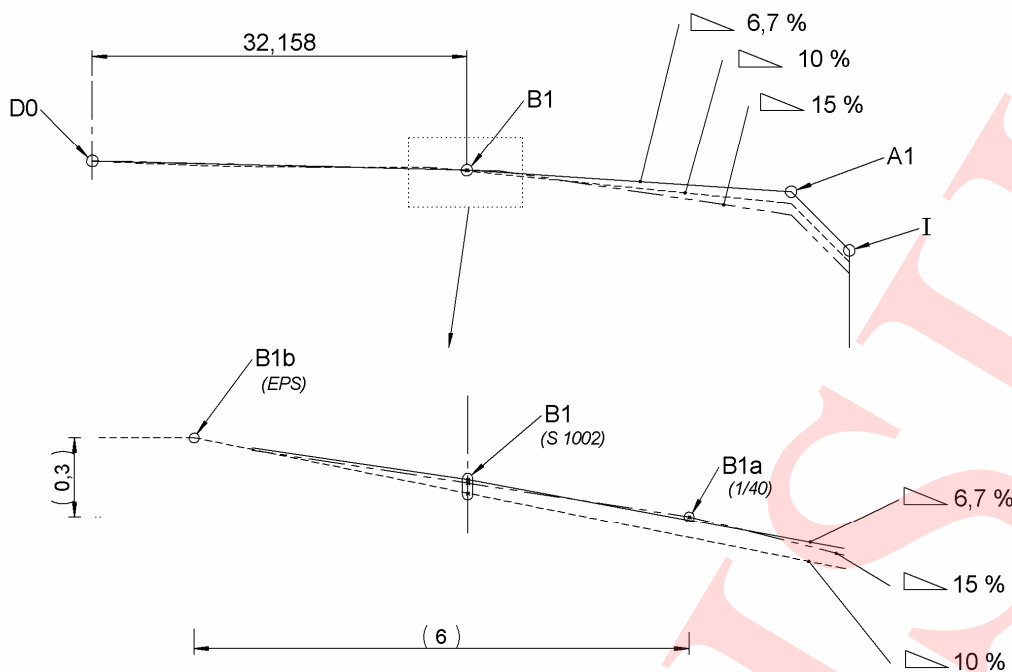
Figure 9 – Reverse slope and chamfer
